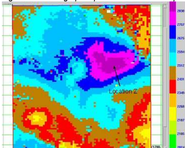
Fig 5. Slice through pore pressure volume at top reservoir.
